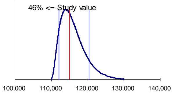
Gamma Left distribution
