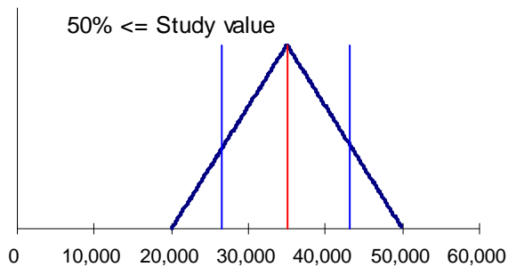
Triangular distribution
